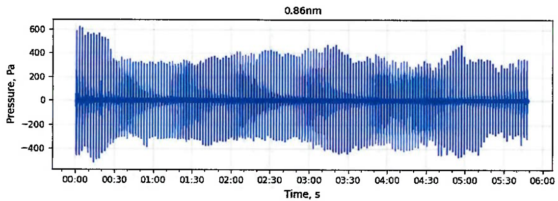
Figure 14. Time series sound pressure, Pa 2:09 pm, 0.86 NM (1.59 km). Pile driving dominant, 160 hammer blows recorded. Orion and support ship propulsion and thruster noise are highly audible (hydrophone through headphones).
