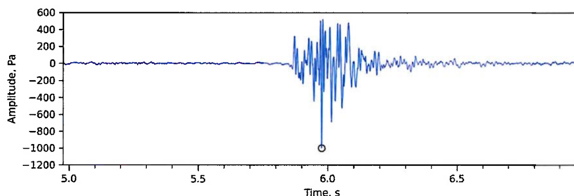
Figure 18. Time series sound pressure, Pa at the highest hammer blow peak at 0.57 NM (1.06 km). Hammer blow signal shows echo/reflection groups and multiple sound speed paths characteristic of reflections off bottom and surface and differing sound speed above and below thermocline.
