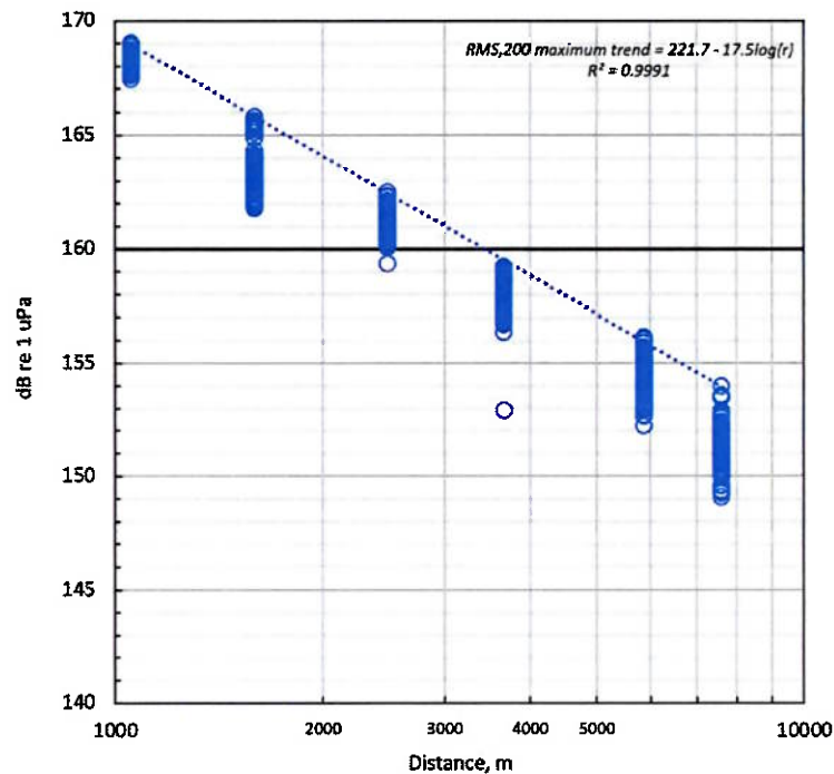
Figure 22. Scatter plot of RMS,200 values for all hammer blows during the survey, with trend of maximum levels for each location.
