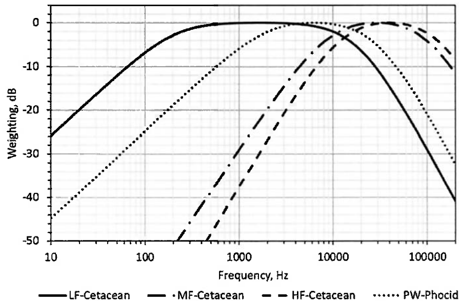
Figure 9. Bode diagram, marine species auditory weightings computed from NMFS 2018.
