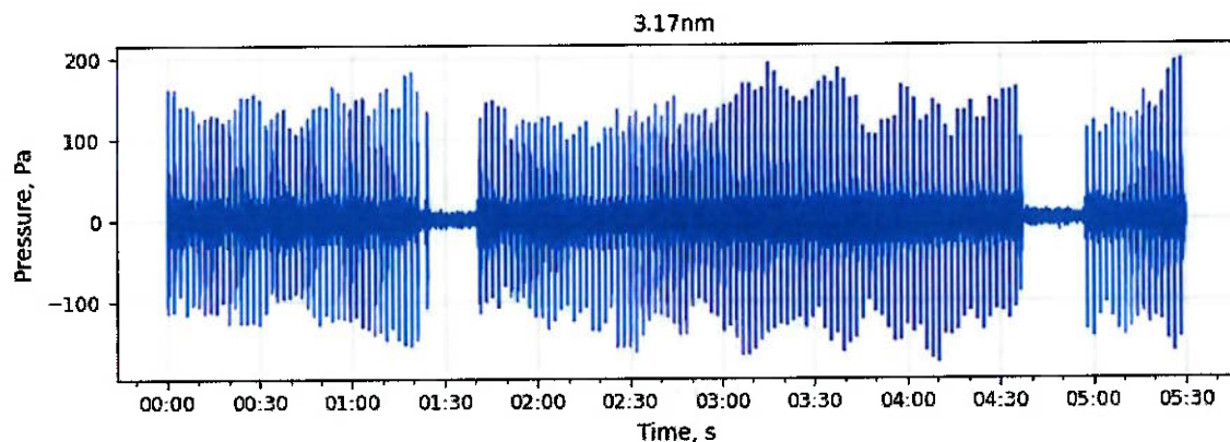
Figure 11. Time series sound pressure, Pa 1:45 pm, 3.17 NM (5.87 km). Pile driving dominant, 146 hammer blows recorded. Orion and support ship propulsion and thrusters are highly audible (hydrophone through headphones). The recording captured two stops with 20-second segments with no hammer blows. Ramp-up was not observed during the two pile driving startups.
