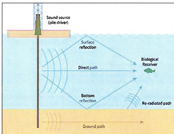
Figure 4. Sound propagation paths associated with pile driving (adapted from Buehler et al., 2015), from BOEM [8].
