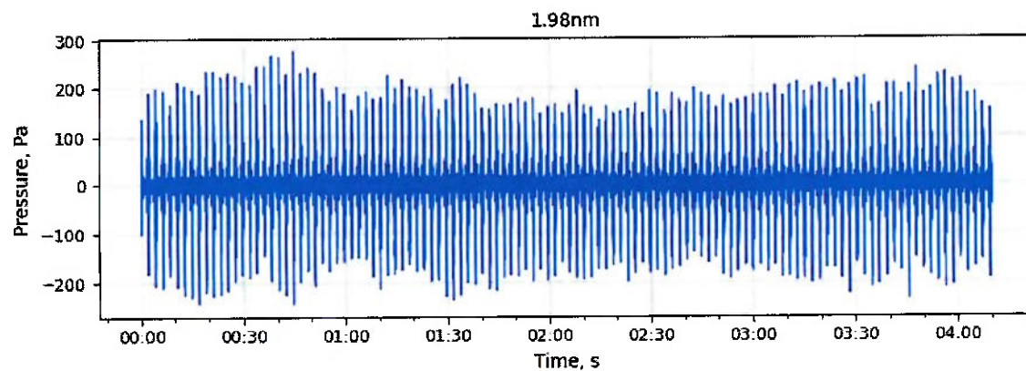
Figure 12. Time series sound pressure, Pa 1:59 pm, 1.98 NM (3.67 km). Pile driving dominant, 117 hammer blows recorded. Orion and support ship propulsion and thruster noise are highly audible (hydrophone through headphones).
