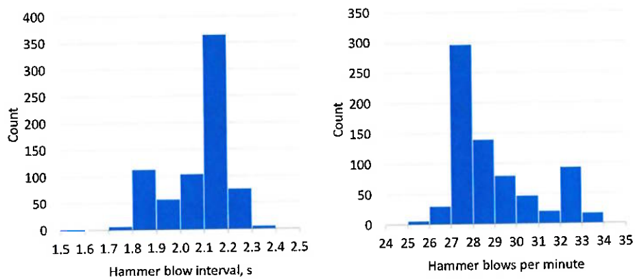
Figure 17. Histograms, hammer blow interval, seconds and blows per minute.
