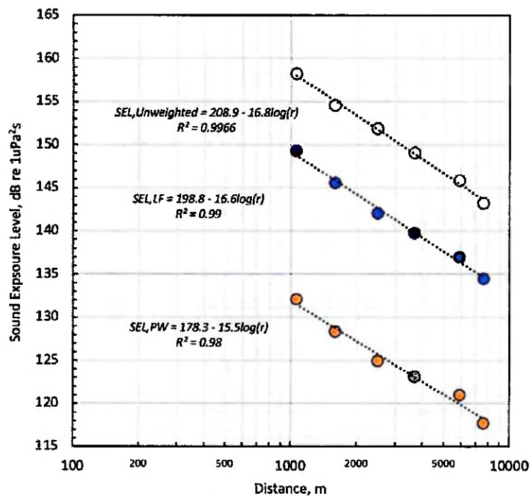
Figure 34. Sound exposure SEL values for unweighted, LF and PW weightings.
