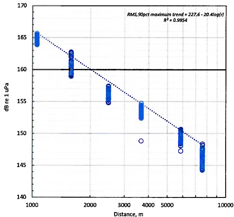
Figure 23. Scatter plot of RMS,90pct values for all hammer blows during the survey, with trend of maximum levels for each location.
