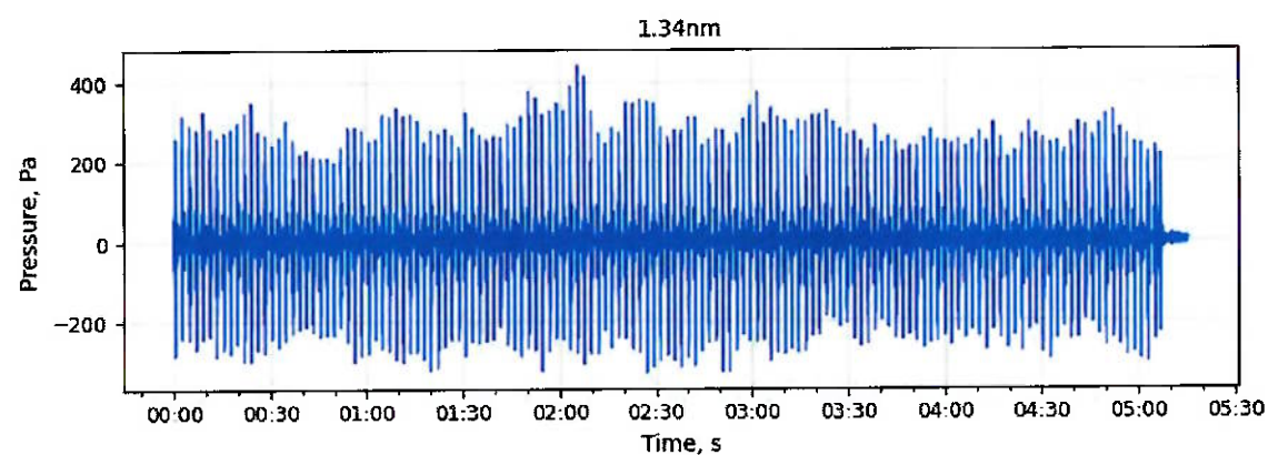
Figure 13. Time series sound pressure, Pa 2:09 pm, 1.34 NM (2.48 km). Pile driving dominant, 143 hammer blows recorded. Orion and support ship propulsion and thruster noise are highly audible (hydrophone through headphones).
