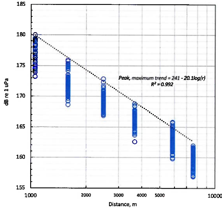
Figure 20. Peak values for all hammer blows during the survey. Lpk Source Level (SLpk) conservatively estimated with highest occurring peaks at each location/.
