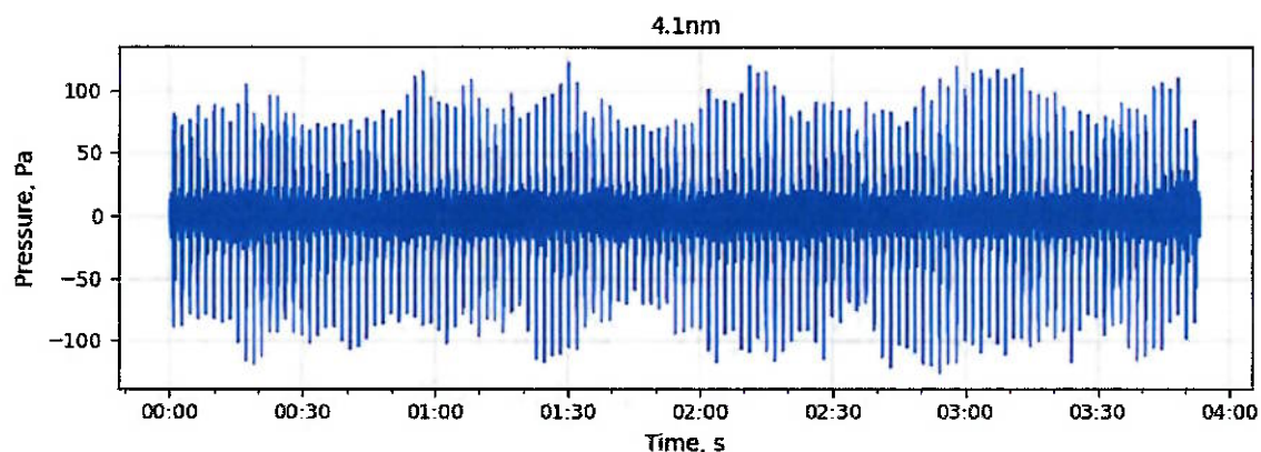
Figure 10. Time series sound pressure, Pa 1:36 pm, 4.1 NM (7.59 km). Pile driving dominant, 126 hammer blows recorded. Orion and support ship propulsion and thruster noise are highly audible (hydrophone through headphones).
